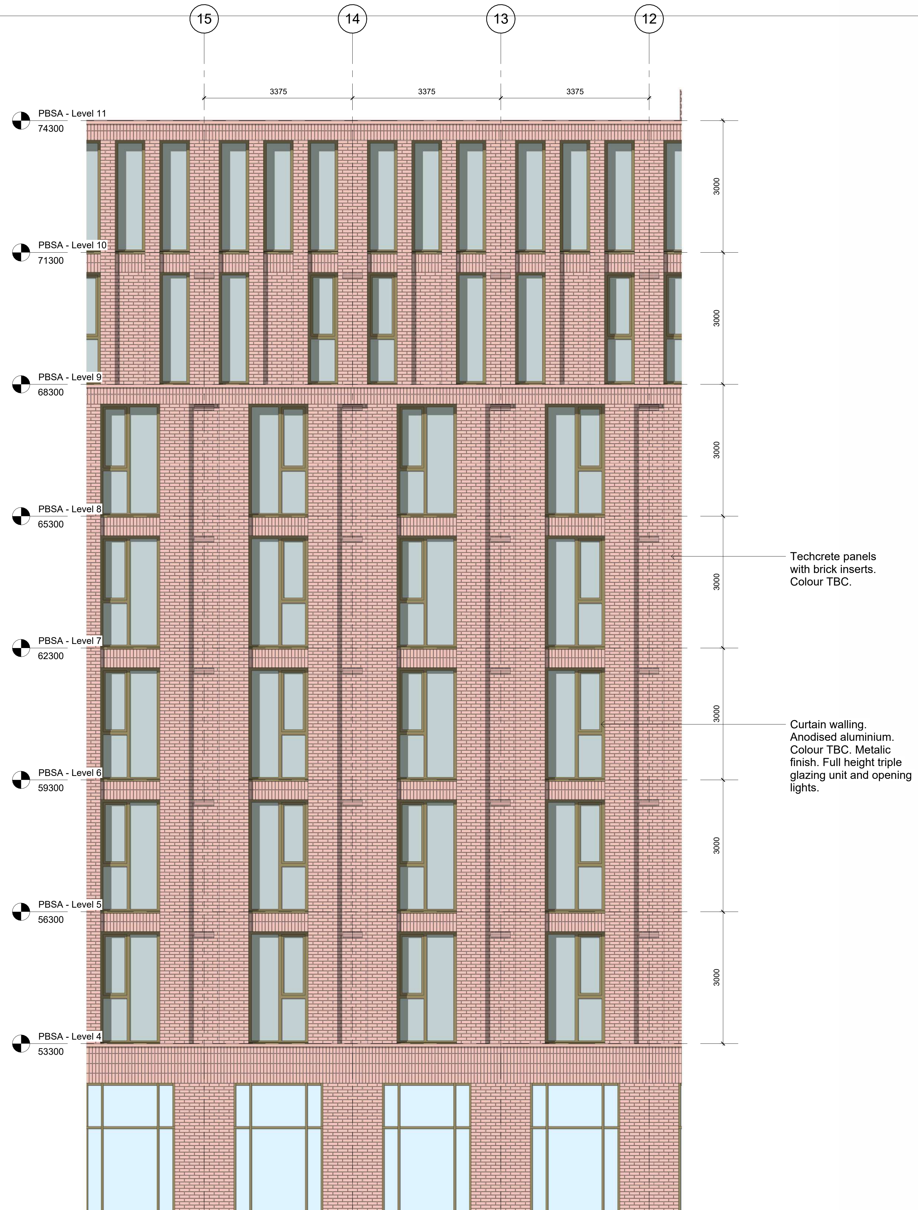
Proposed PBSA Elevation Bay Details 1 1 : 50
