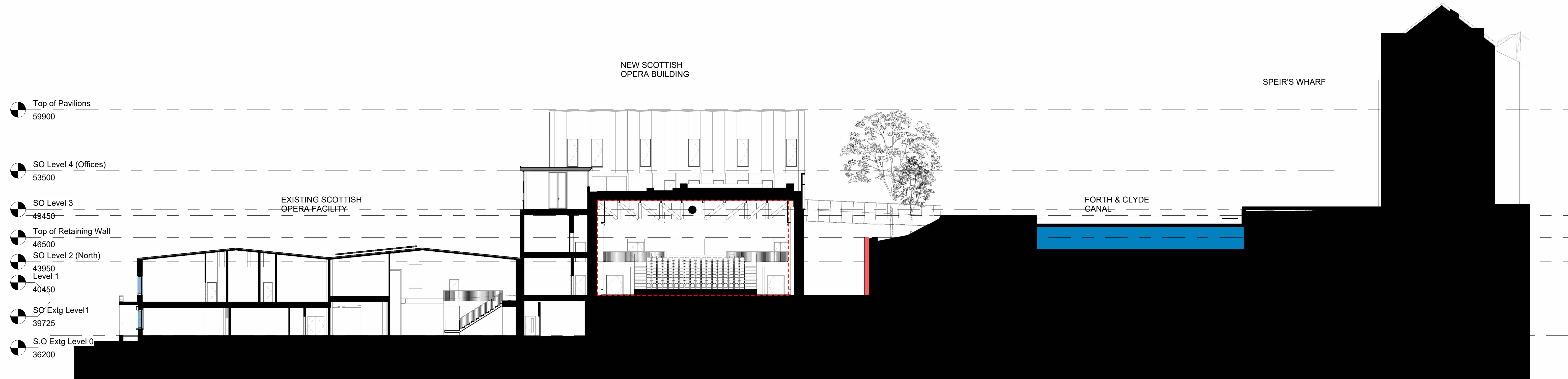
2 Scottish Opera cross section B-B 1 : 200
