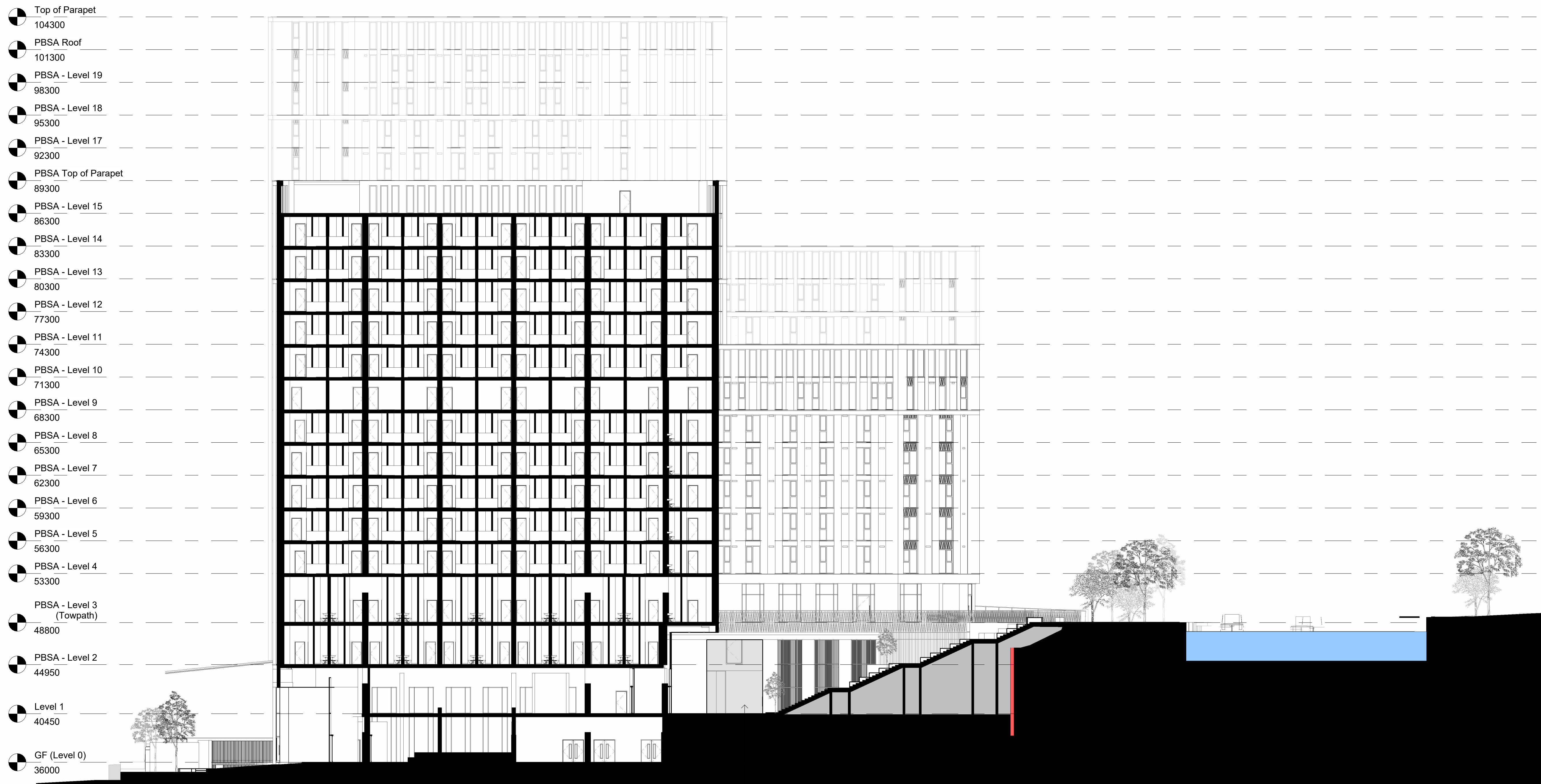
PBSA South - Section B-B 1 : 200
