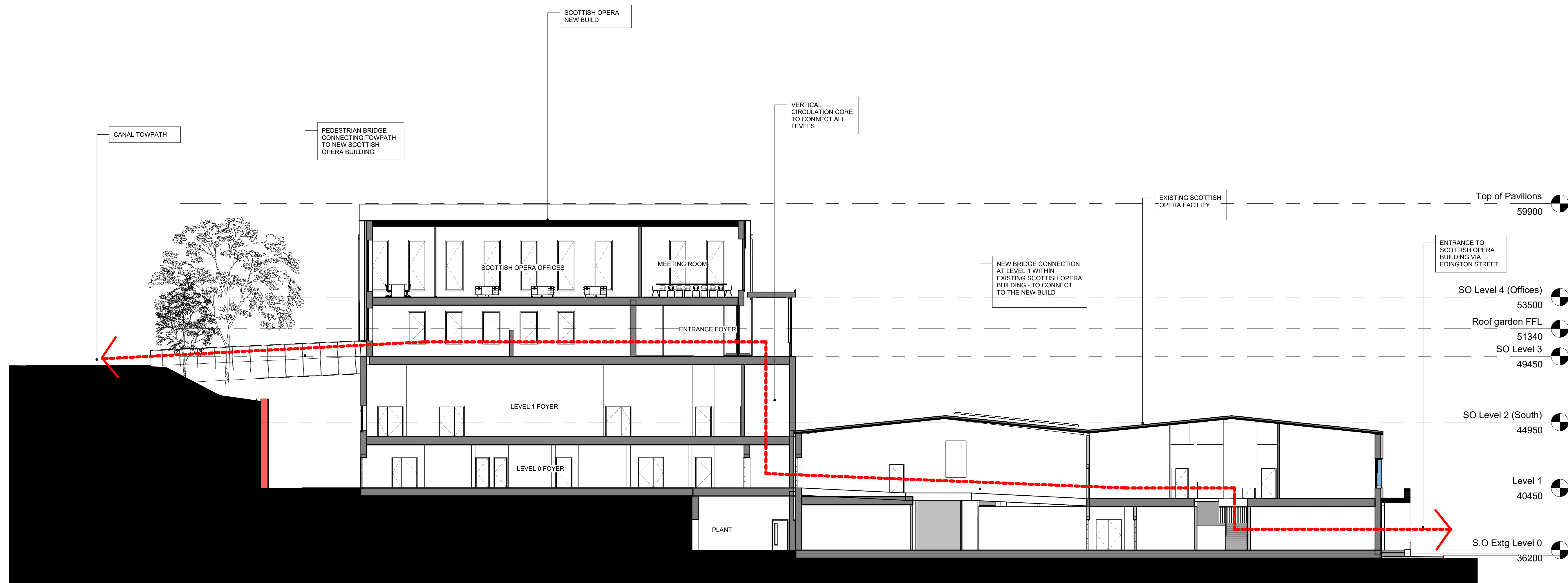
1 Scottish Opera cross section E-E (connection through) 1 : 150
