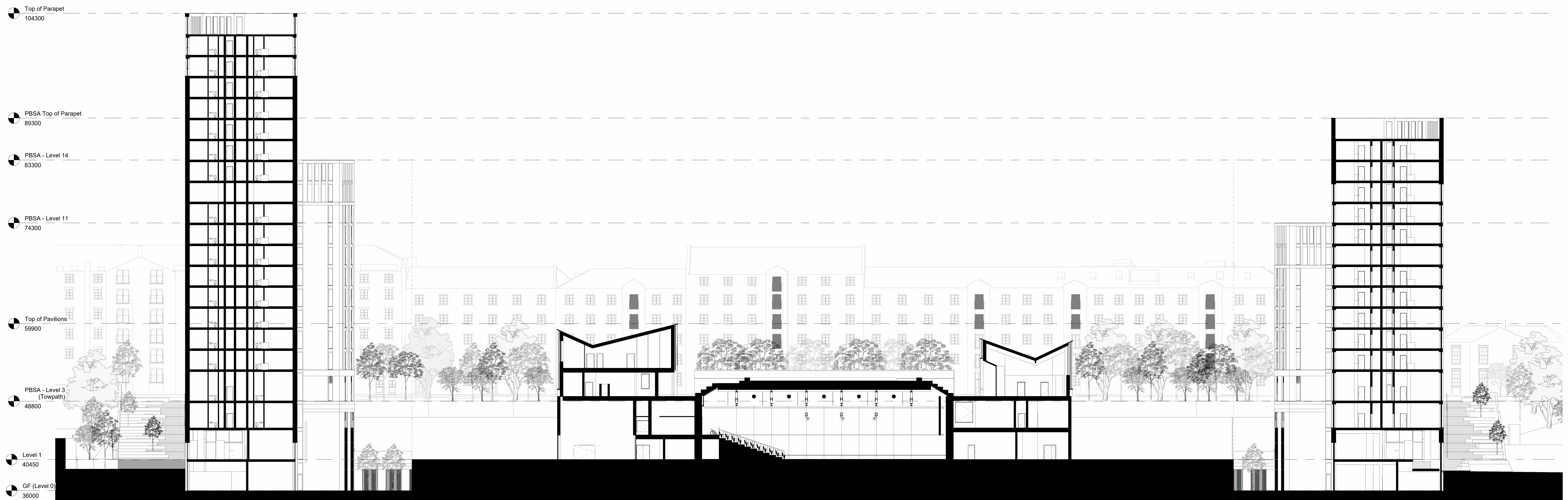
Proposed Site Section C-C 1 : 200
