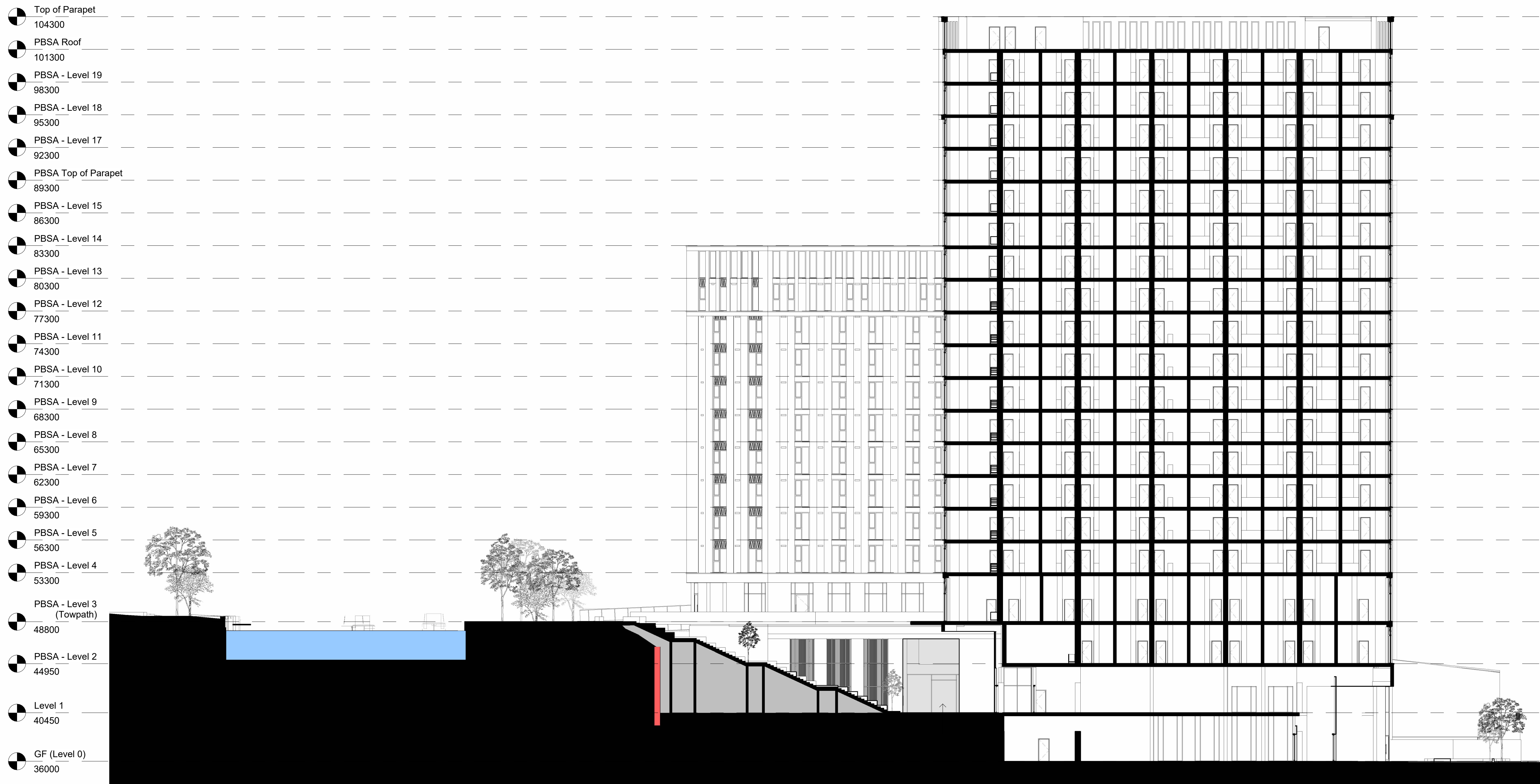
PBSA North - Section A-A 1 : 200
