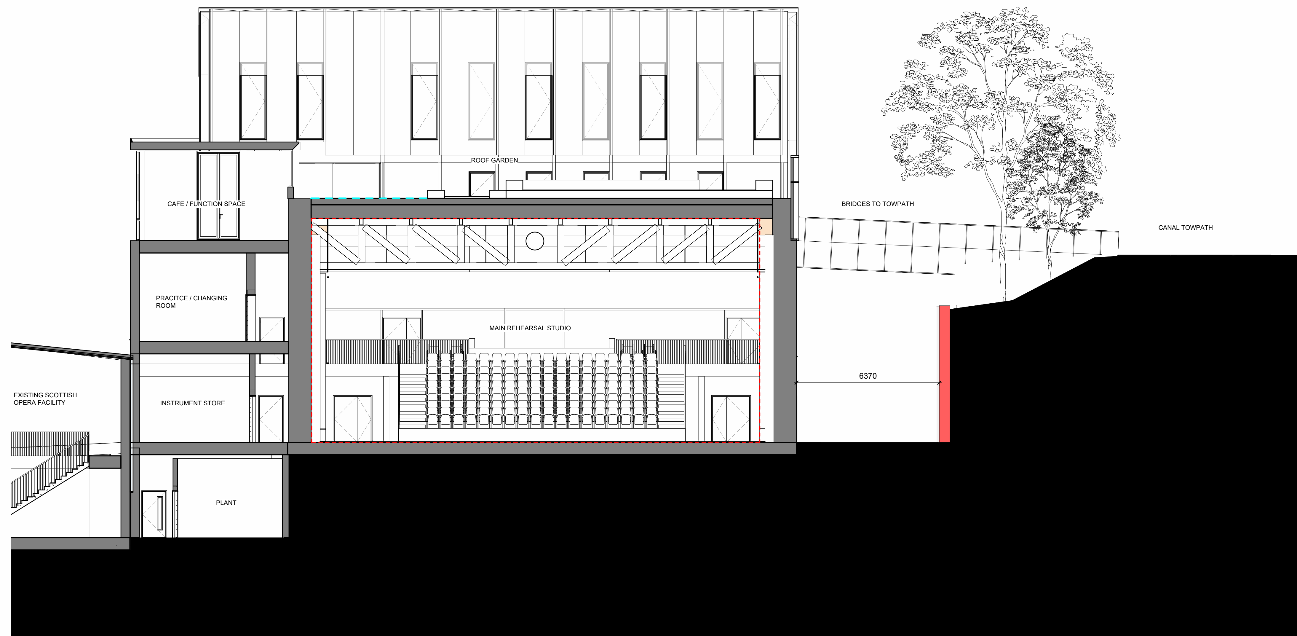
1 Scottish Opera cross section B-B (Thru' main studio) 1 : 100
