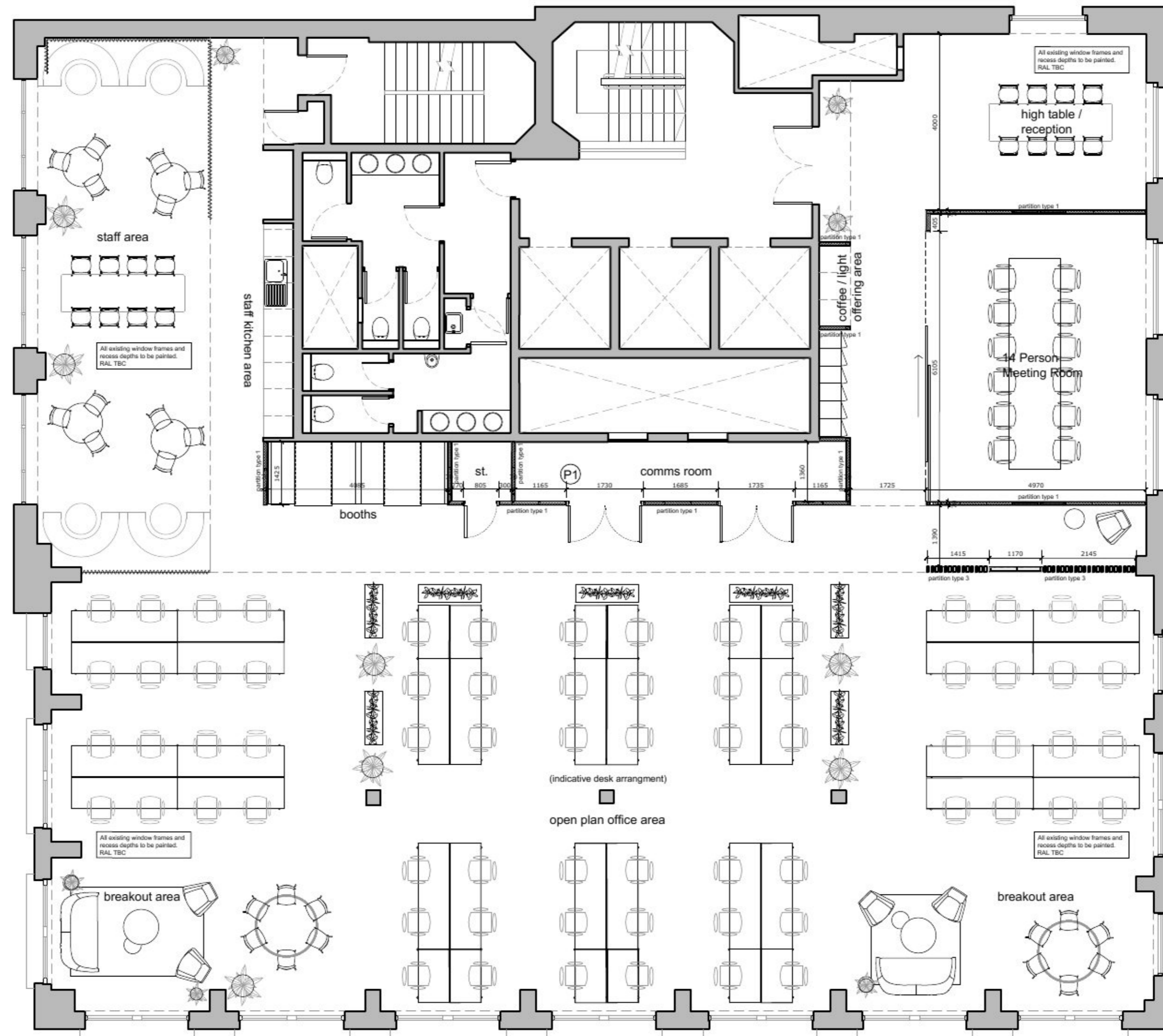
Proposed Layout
