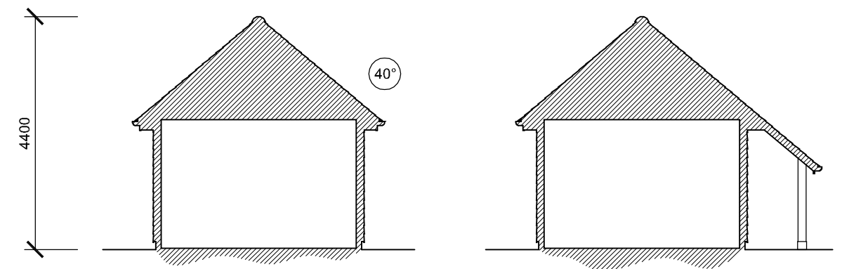
Cross Sections
