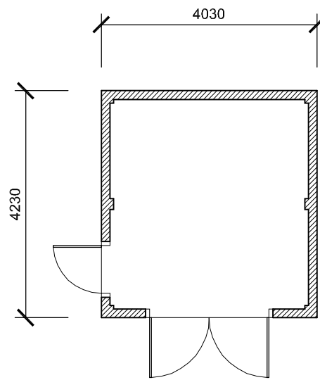
Floor Plan
