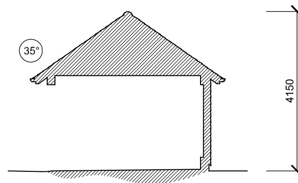
Cross Section
