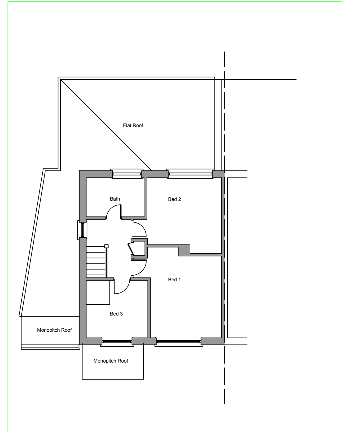
Proposed First Floor + Roof of Extension
