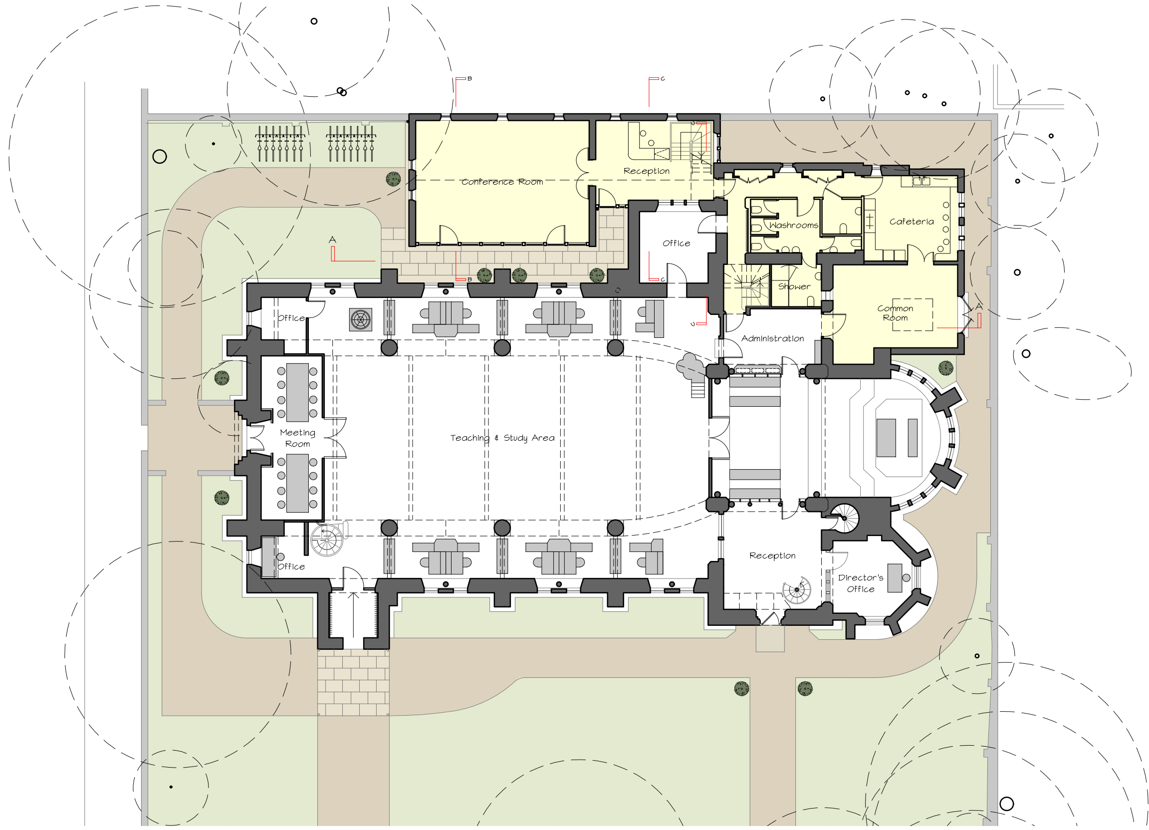
GROUND FLOOR AS PROPOSED SCALE 1:200 AT A3
