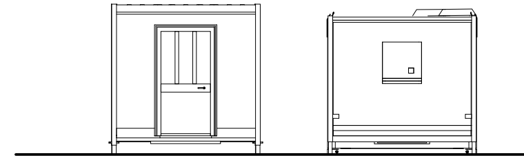
West Elevation
