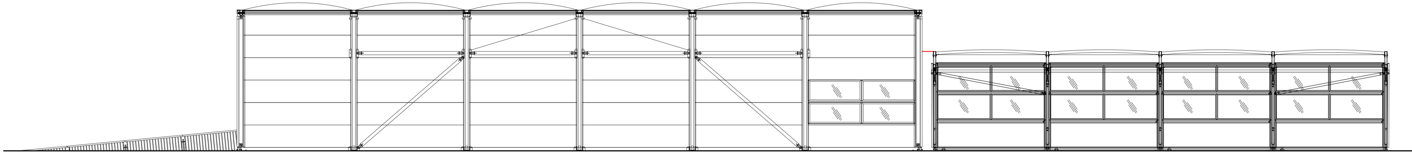
Marquee East Elevation
