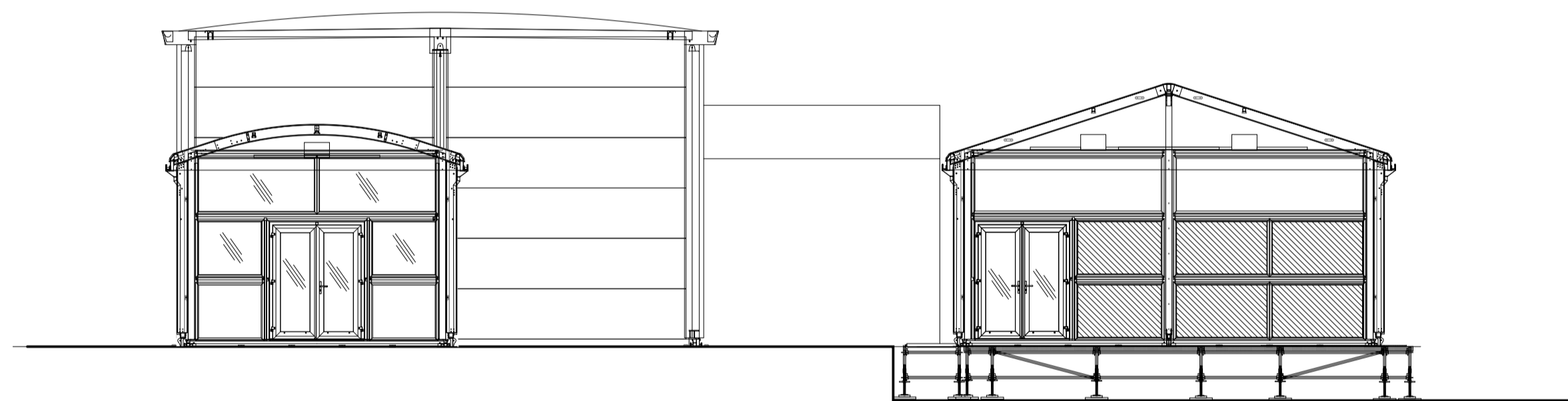
Marquee North Elevation
