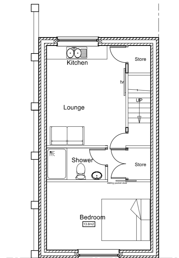
FIRSTFLOOR (PROPOSED)
