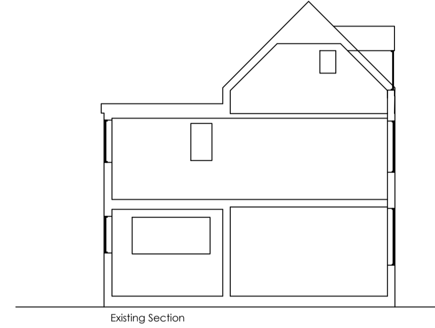
Existing Section
