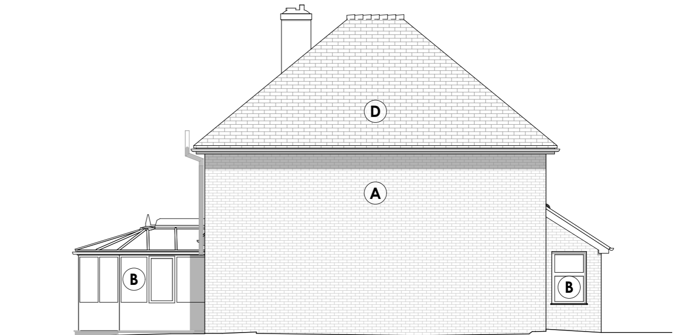
South-East Elevation
