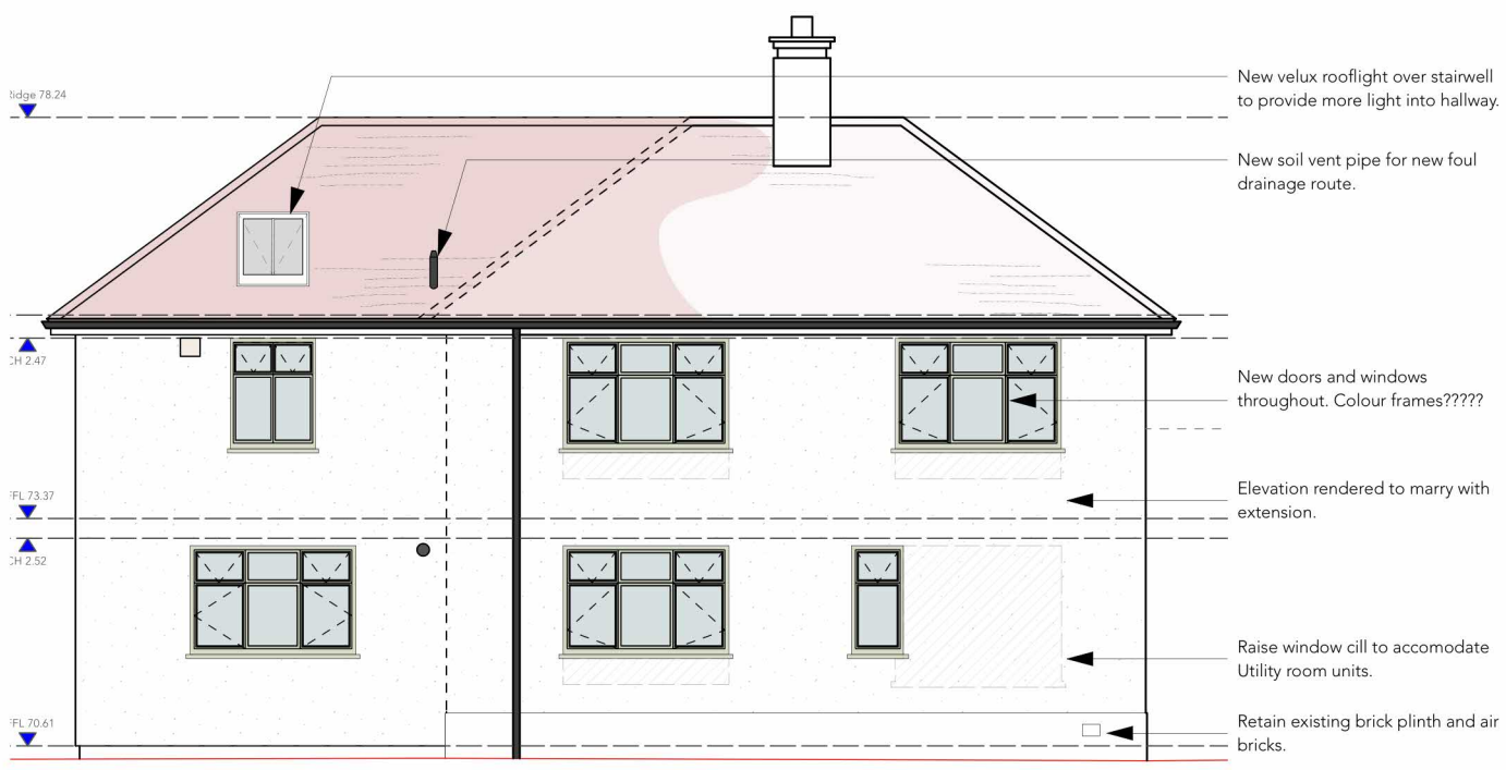
East Elevation
