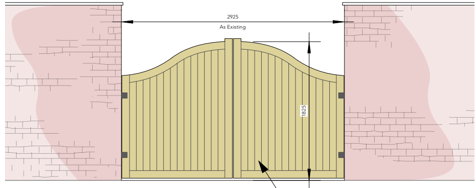
Gate Elevation
