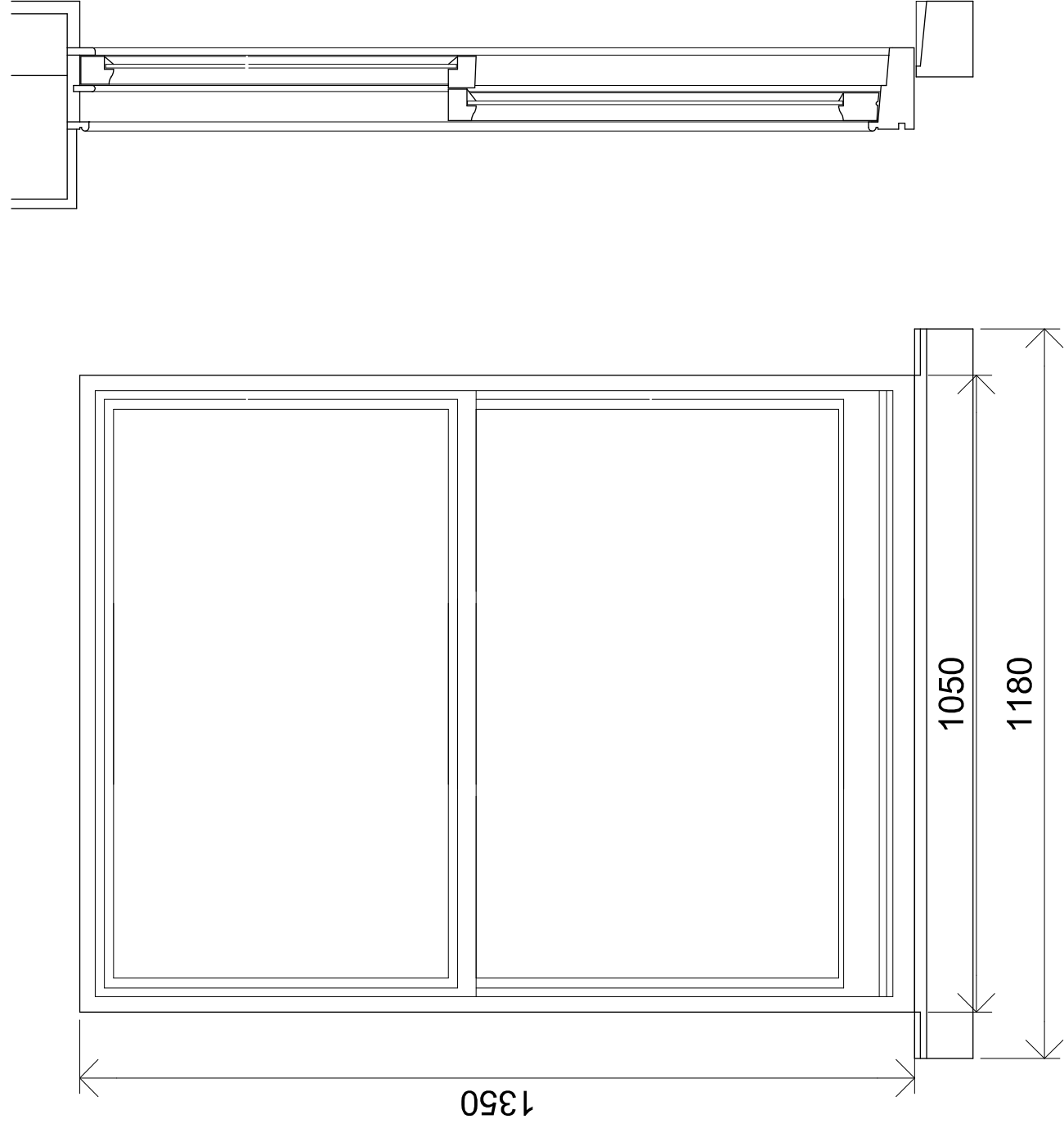
EXTERNAL ELEVATION
