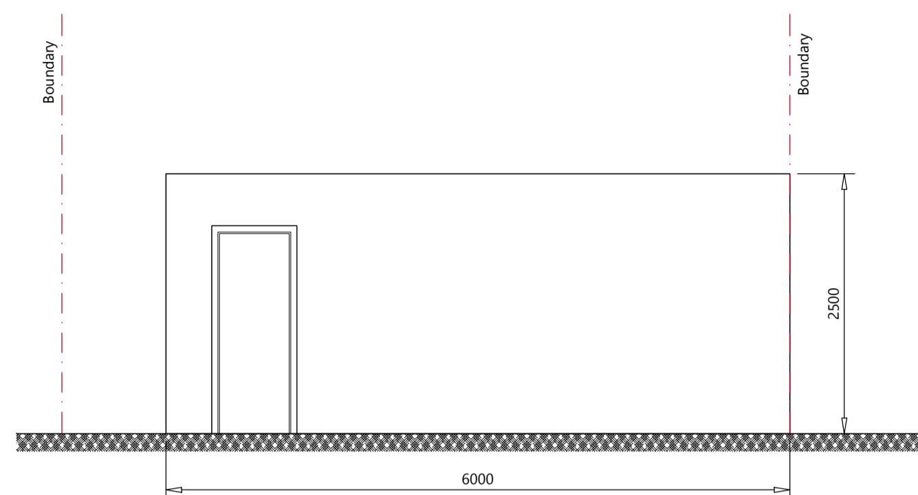
ELEVATION A-A SCALE 1:50
