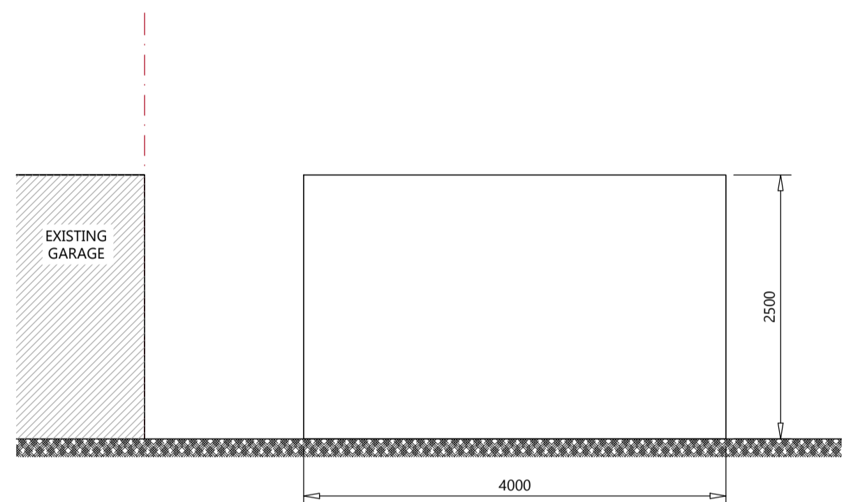
ELEVATION B-B SCALE 1:50
