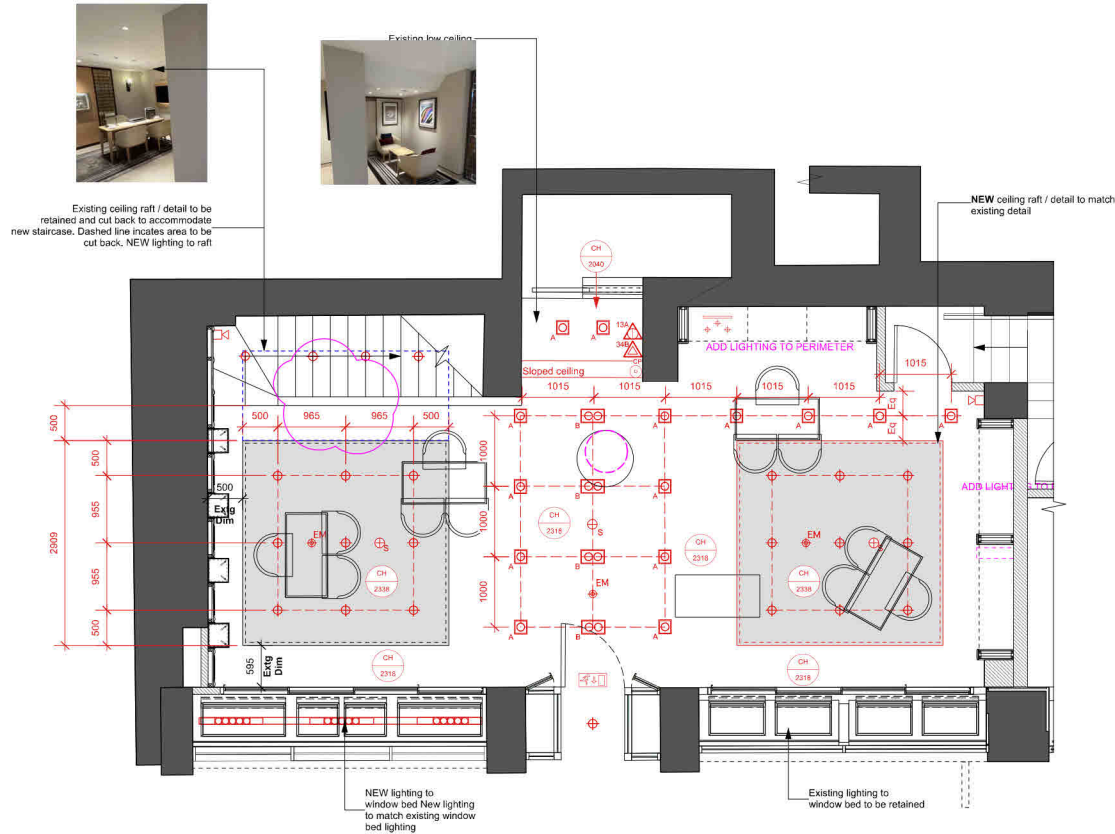
01 GROUND FLOOR RCP LAYOUT Scale: 1:50
