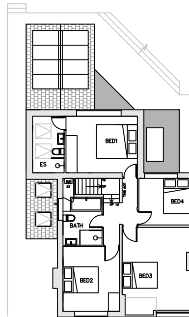
PROPOSED FIRST FLOOR
