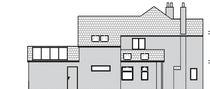
PROPOSED SIDE ELEVATION WEST FACING
