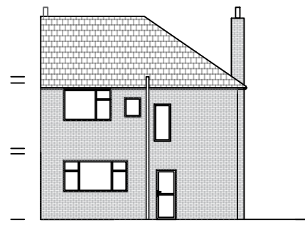
EXISTING REAR ELEVATION NORTH FACING
