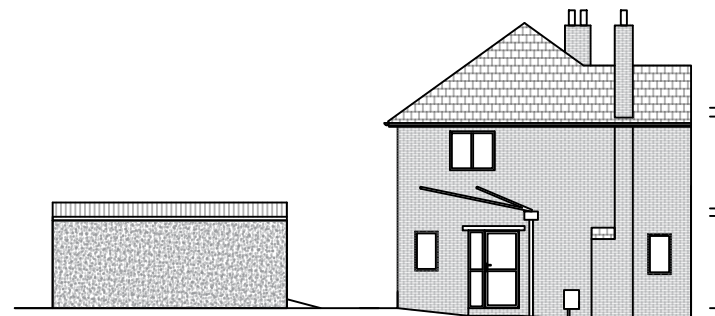
EXISTING SIDE ELEVATION WEST FACING
