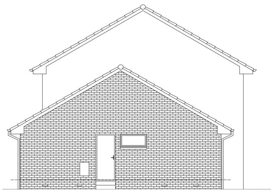
Existing Gable Elevation (1:100)
