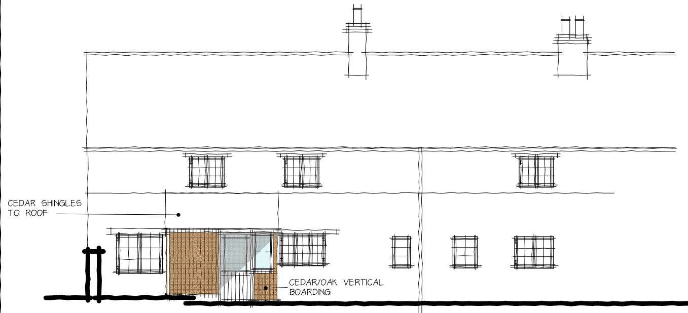
PROPOSED SOUTH WEST ELEVATION
