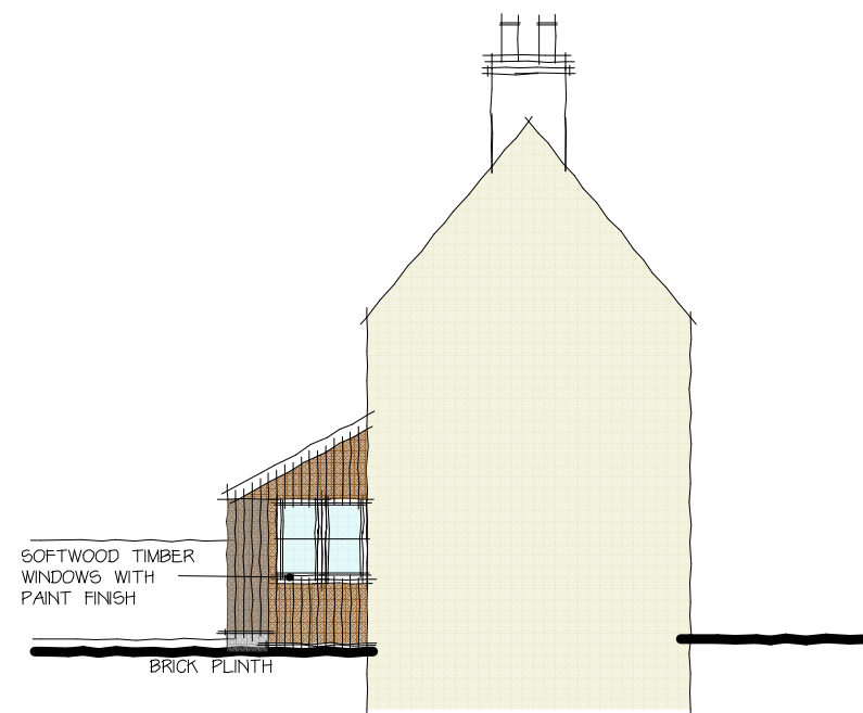
PROPOSED SOUTH EAST ELEVATION
