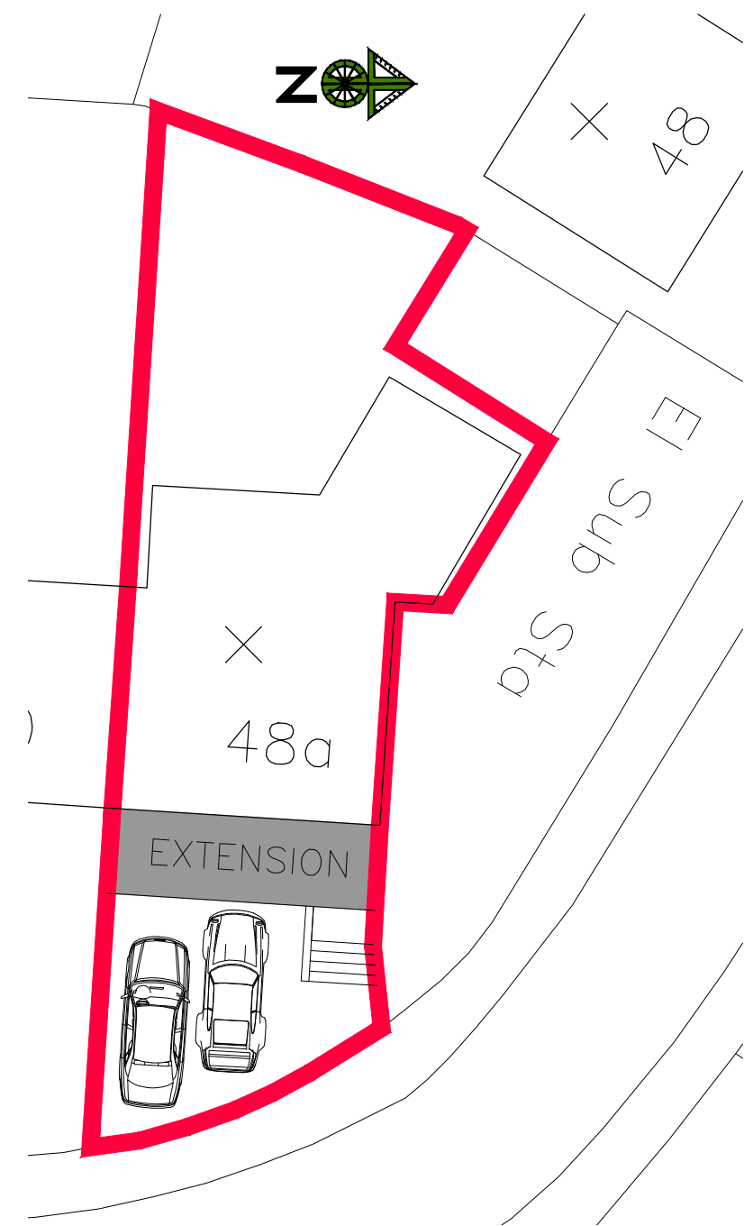
BLOCK PLAN (1:200) 0 4.0 8.0 12.0 16.0 20.0m 1:200
