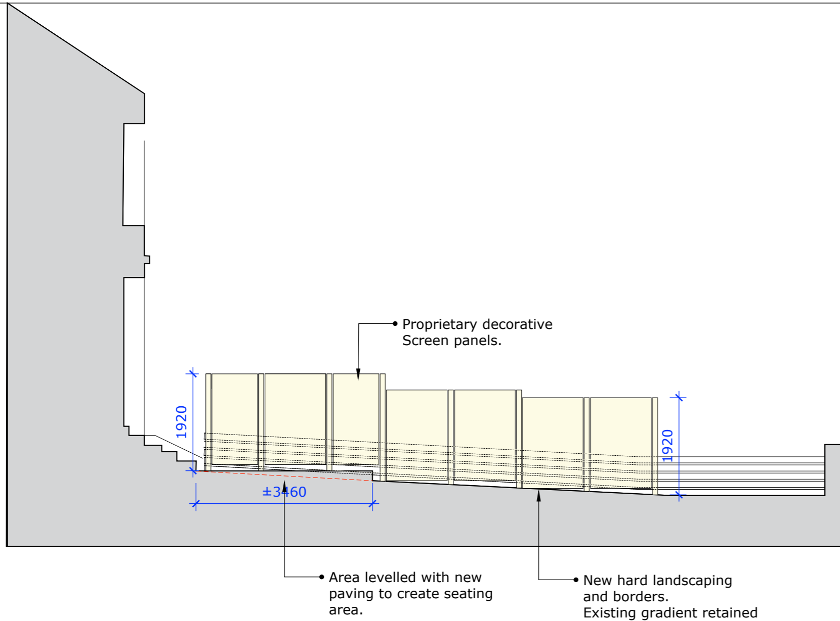
SECTION B 1:75 FRONT GARDEN
