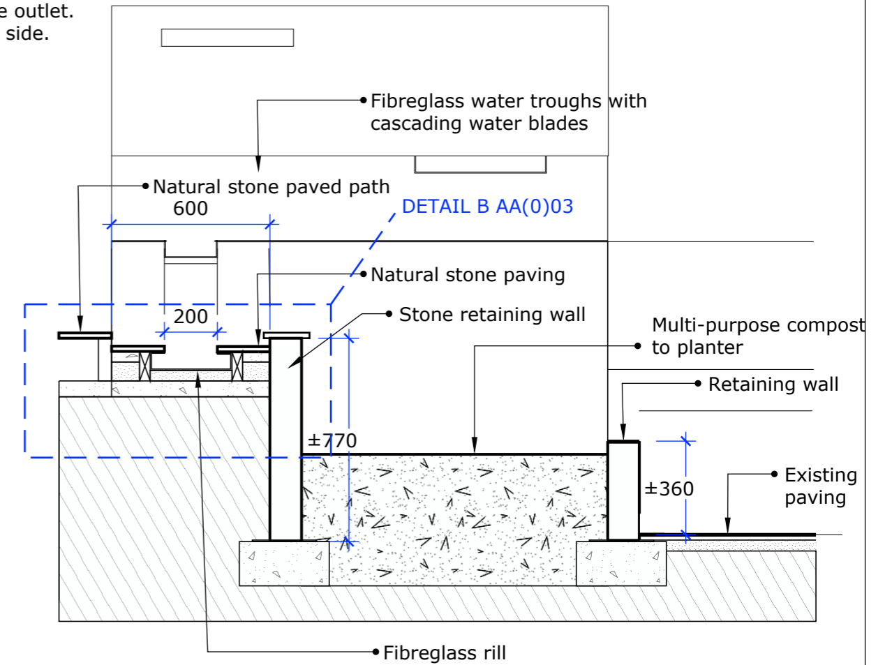
SECTION C-C 1:20
