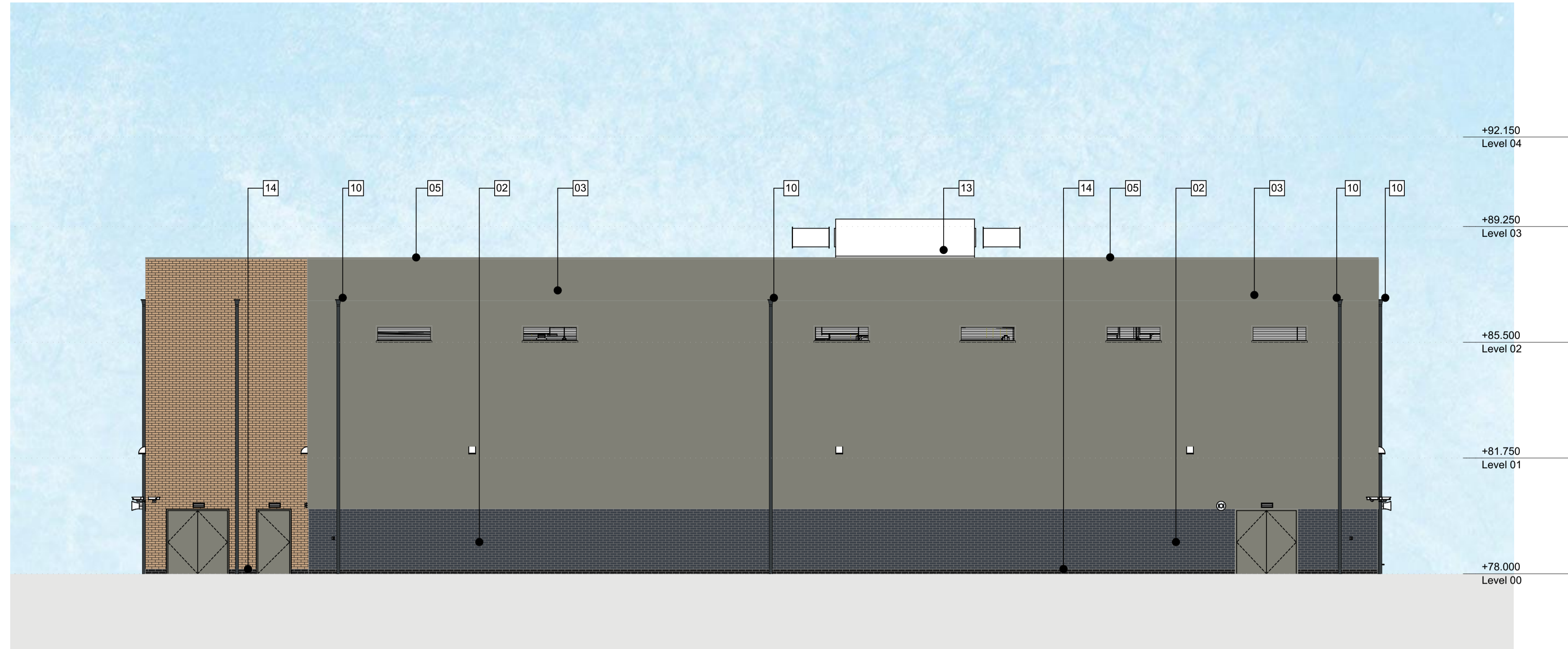
E-05 Elevation 'Hall North' 1:100
