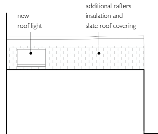
WEST ELEVATION
