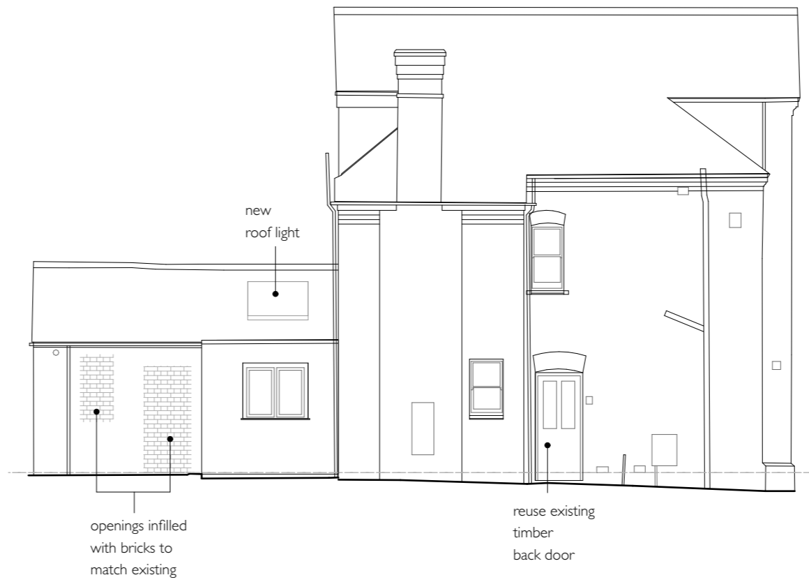
EAST ELEVATION
