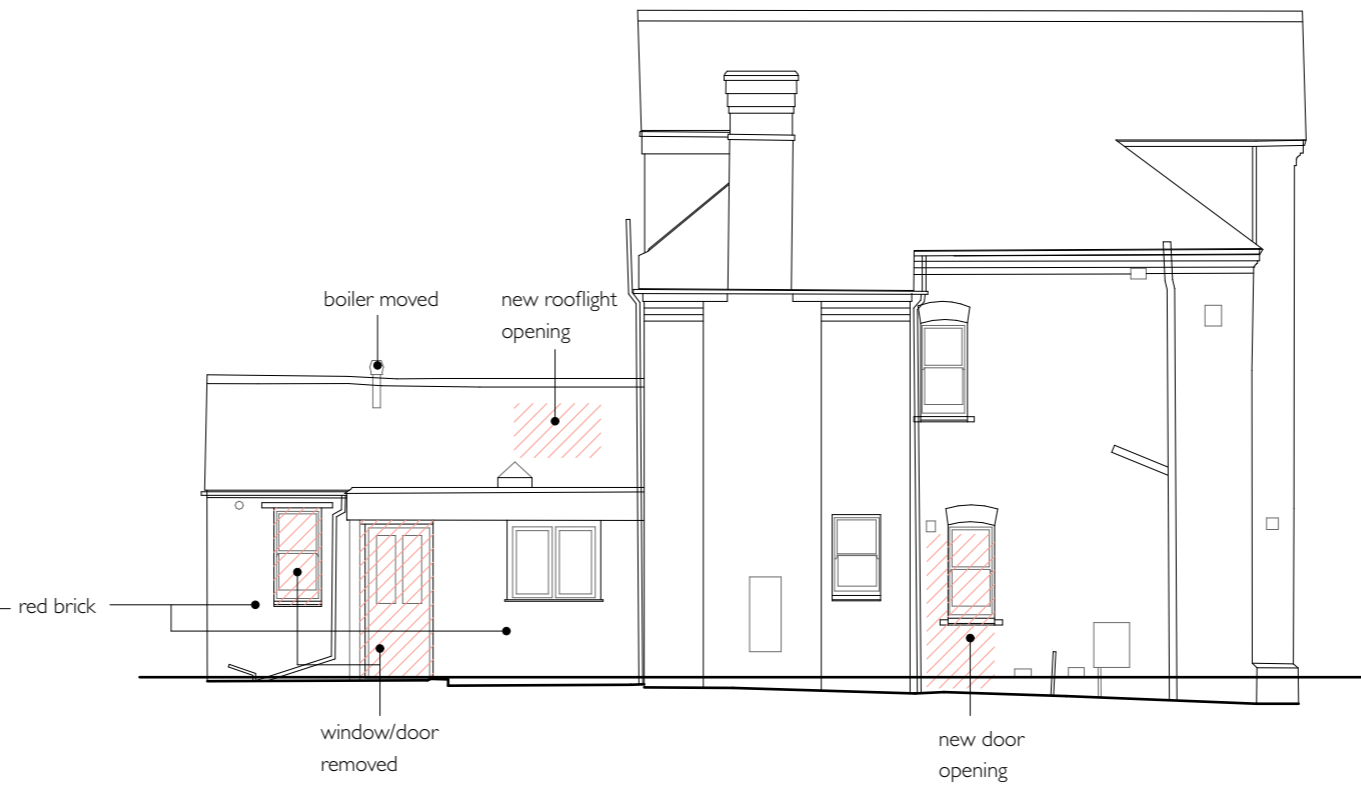
EAST ELEVATION
