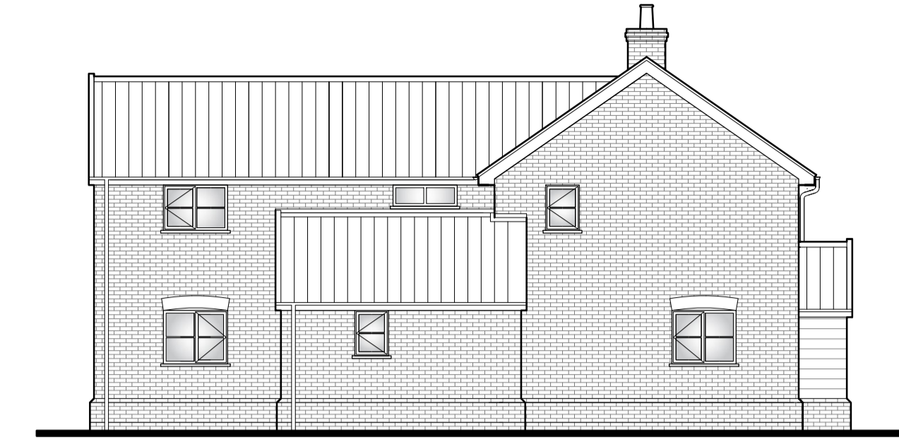
PROPOSED NORTH-EAST SIDE ELEVATION
