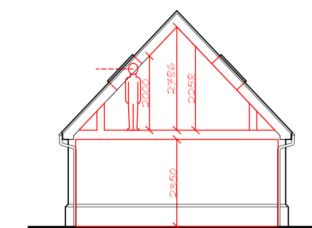
SECTION THROUGH PROPOSED EAST SIDE ELEVATION SHOWING HEAD HEIGHTS
