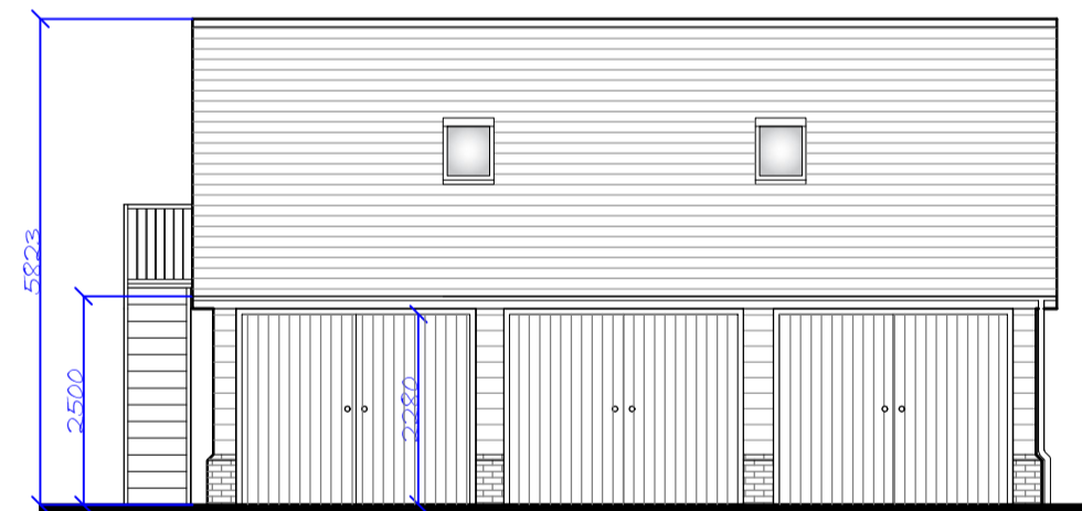
PROPOSED SOUTH FRONT ELEVATION
