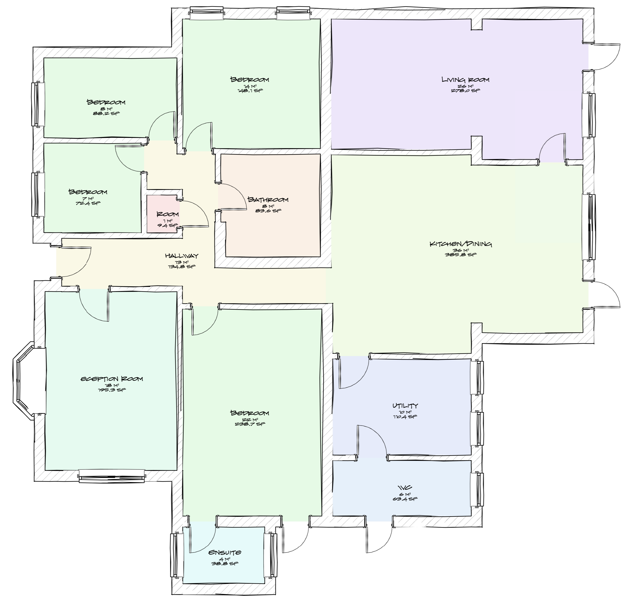
1 GROUND FLOOR 1 : 50
