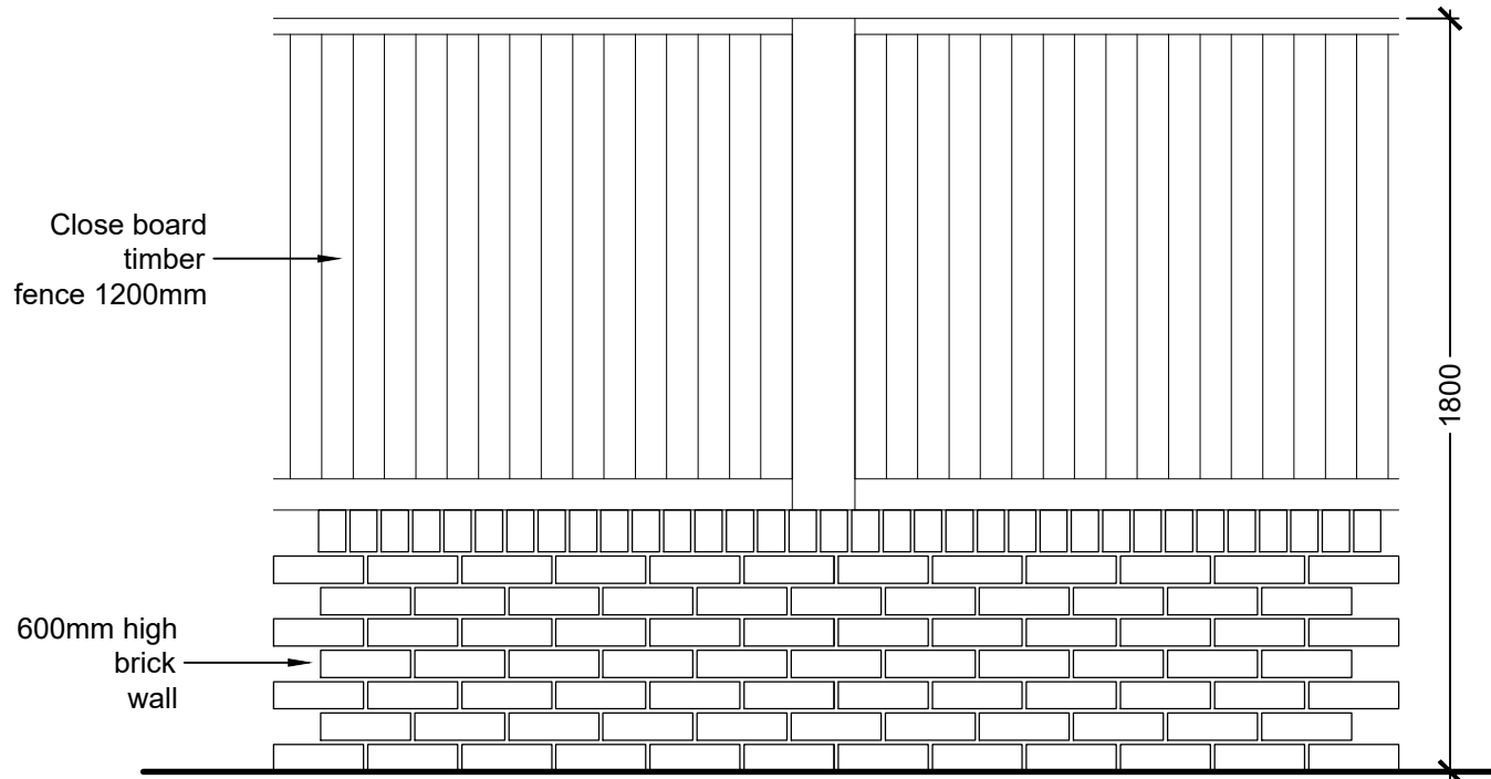
Typical Elevation Wall Detail
