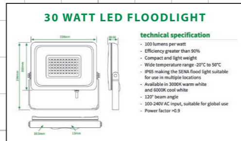
D FOUR X LED FLOOD LIGHTS SIZE. 0.23m x 168mm. H.A.G. 5.6m.
