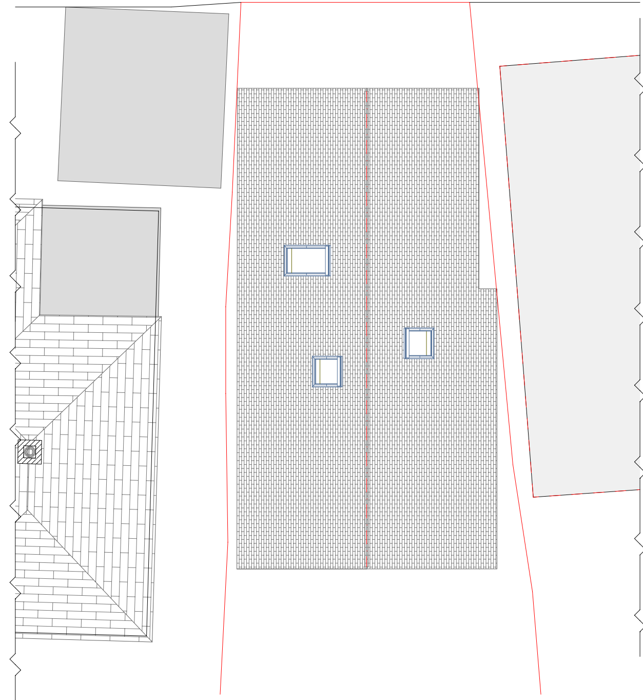
2 Proposed Roof 1:100
