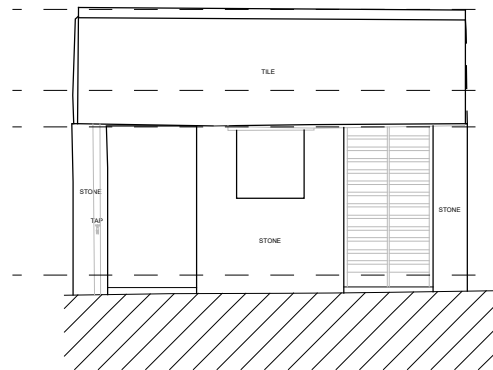
OUTBUILDING 2 - WEST ELEVATION
