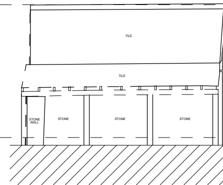
OUTBUILDING 2 - EAST ELEVATION
