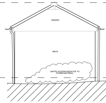
OUTBUILDING 1 - WEST ELEVATION
