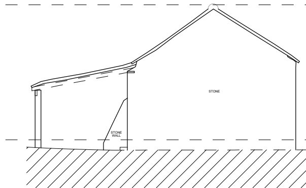
OUTBUILDING 2 - NORTH ELEVATION
