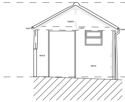
OUTBUILDING 1 - EAST ELEVATION
