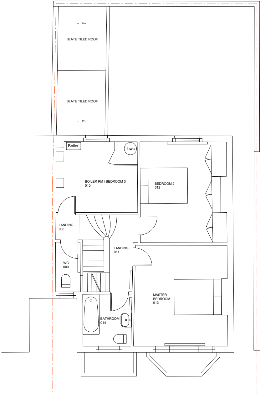
First floor
