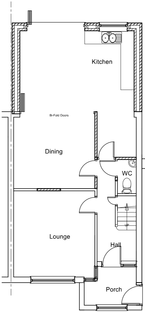
GROUND FLOOR (PROPOSED)
