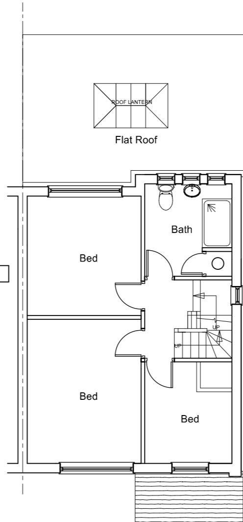
FIRST FLOOR (PROPOSED)
