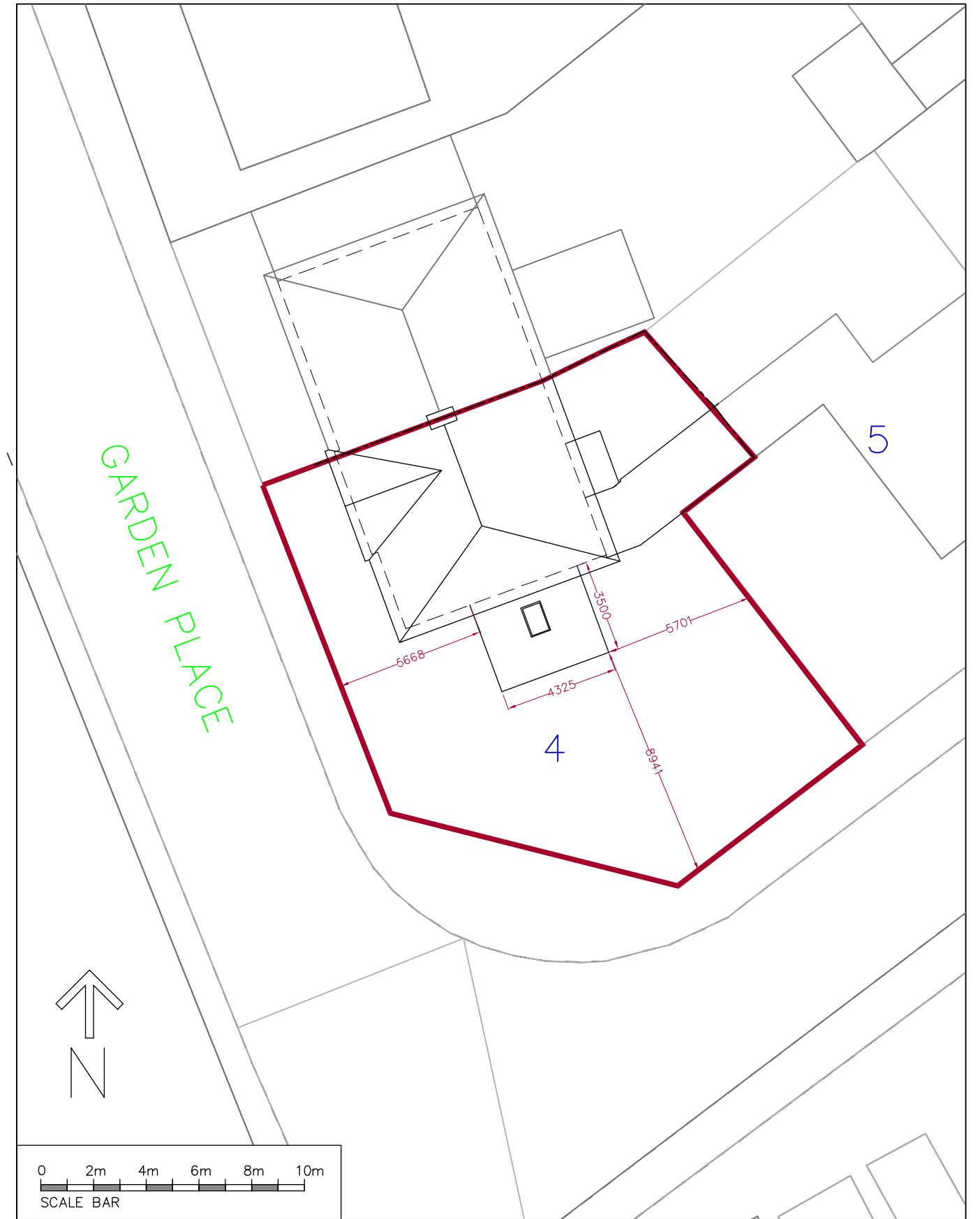
PROPOSED SITE AND ROOF PLAN 1:200
