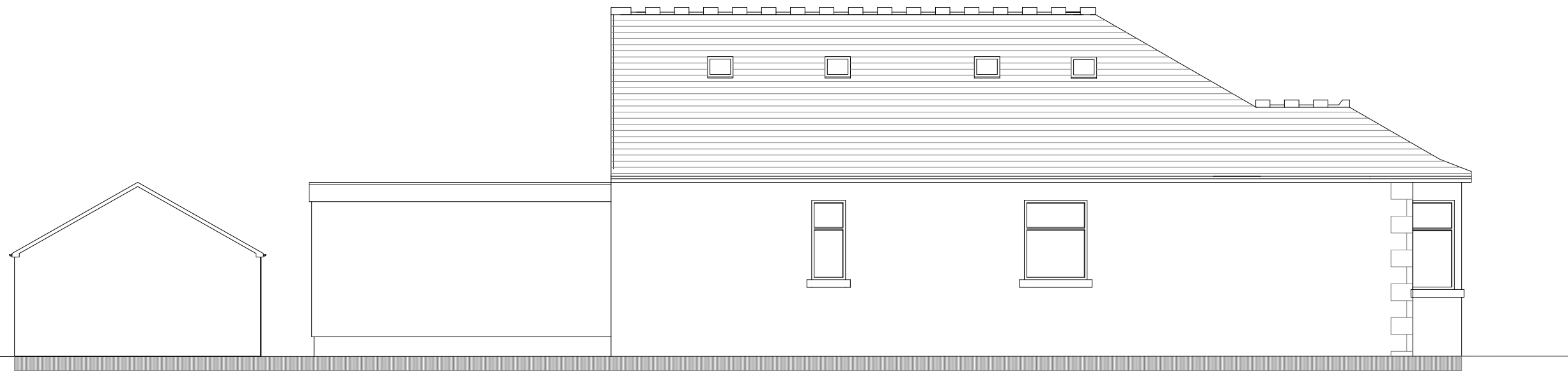
EAST ELEVATION
