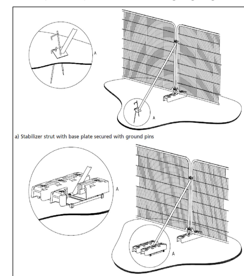
Examples of above-ground stabilising systems (reproduced from BS 5837:2012 Trees in relation to design, demolition and construction - Recommendations)
