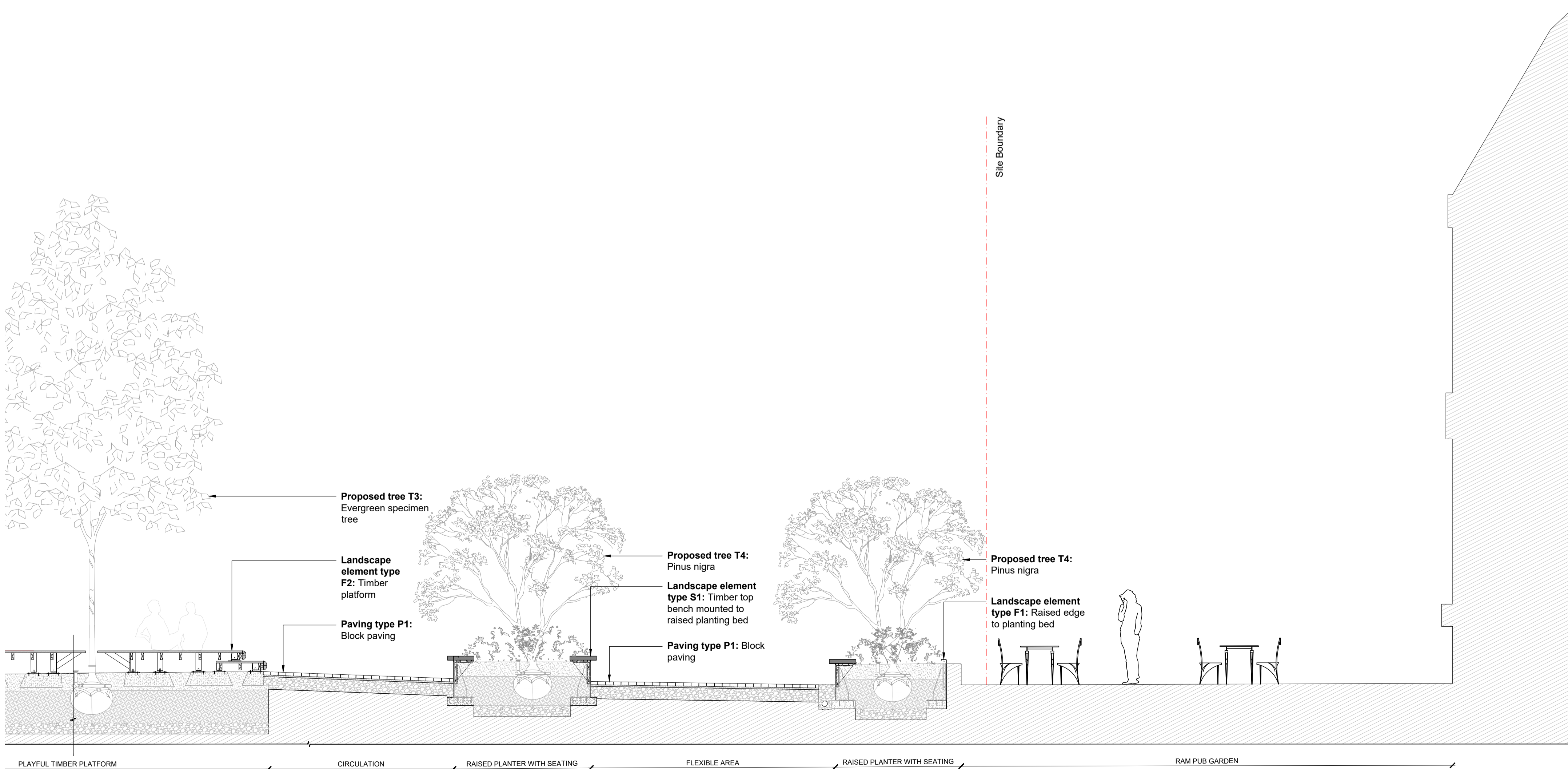
02 SECTION 01 Scale 1:50 @ A1
