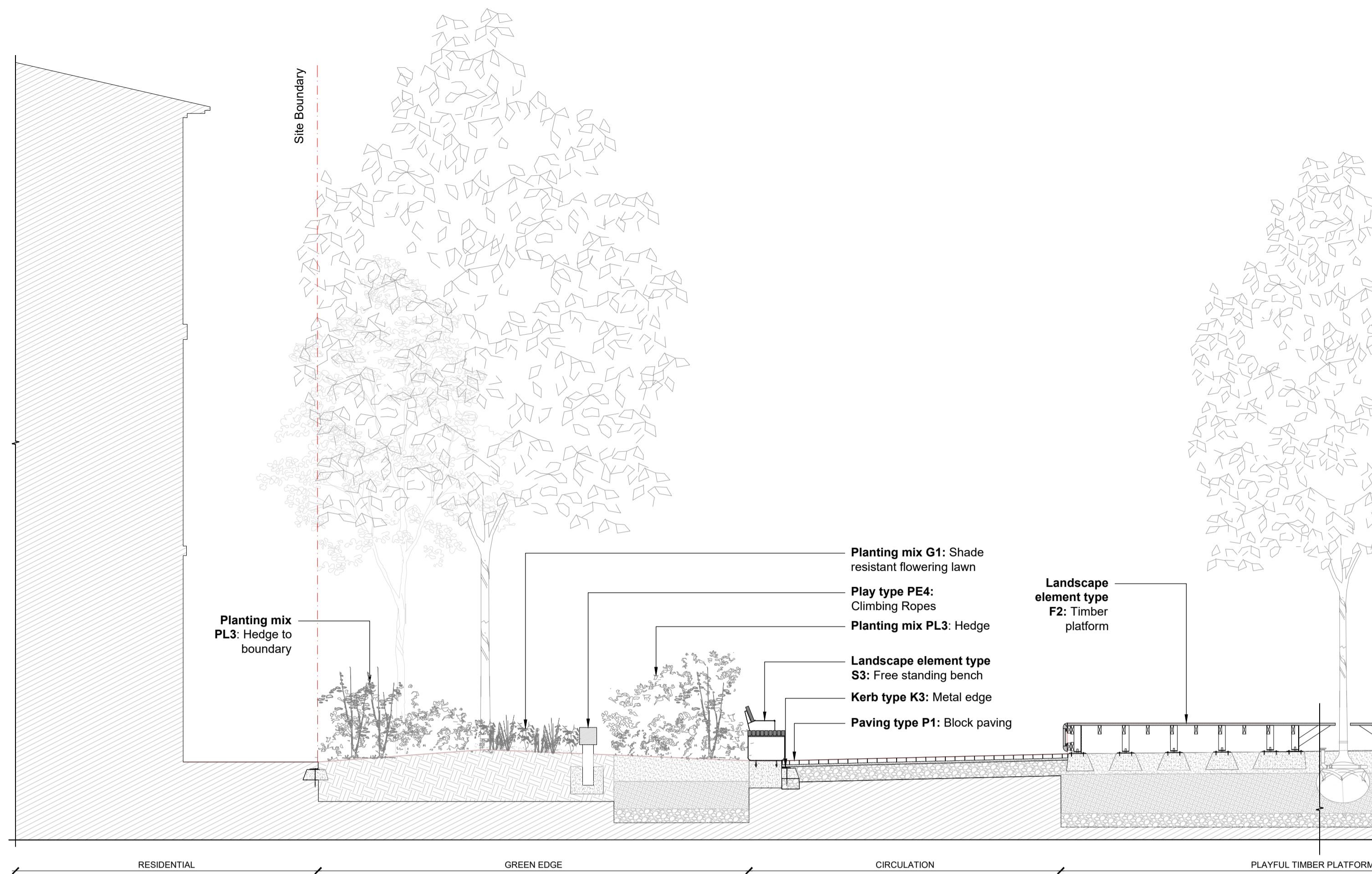
01 SECTION 01 Scale 1:50 @ A1
