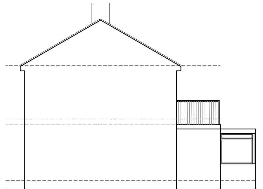
Proposed Sectional Elevation
