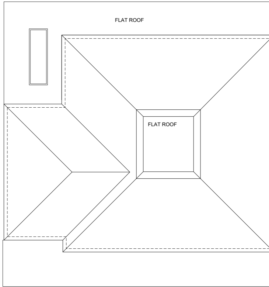
Roof Plan - Proposed
