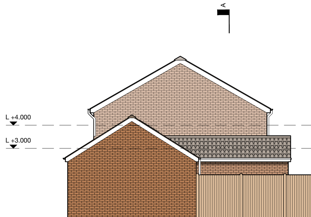
Side West elevation
