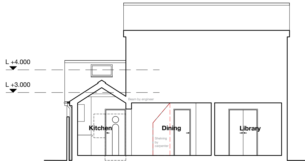
A-A Kitchen, dining and library
