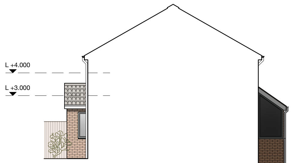
Side East (Sectional elevation)
