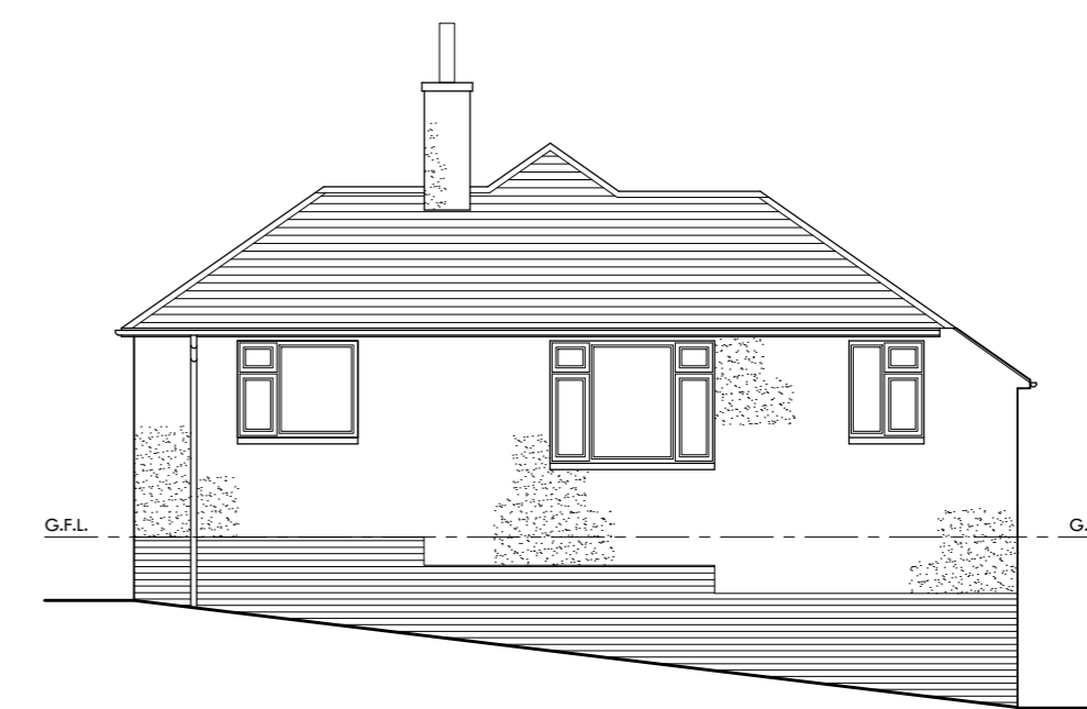
SOUTH EAST ELEVATION 1:100
