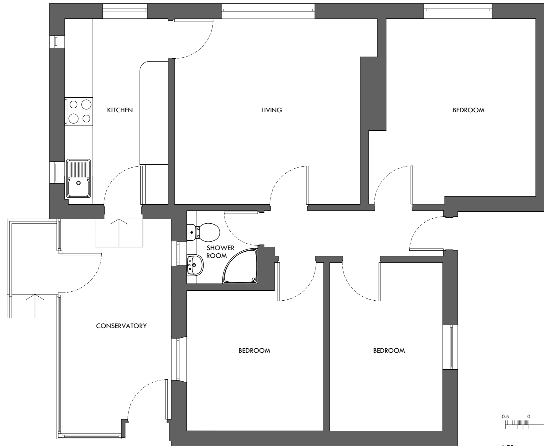
FLOOR PLAN AS EXISTING 1:50
