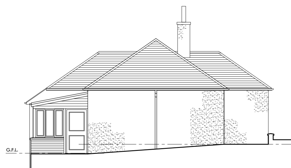
NORTH WEST ELEVATION 1:100
