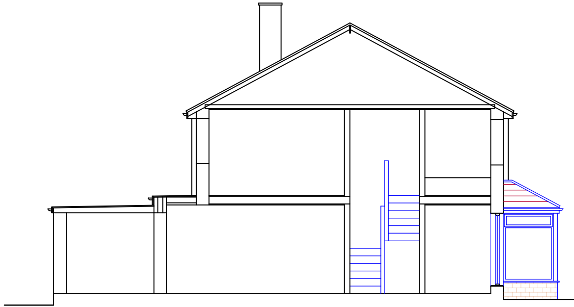
SECTION AS EXISTING
