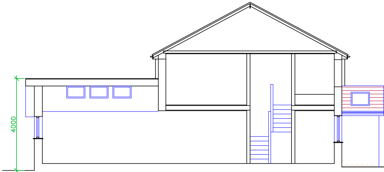
SECTION AS PROPOSED
